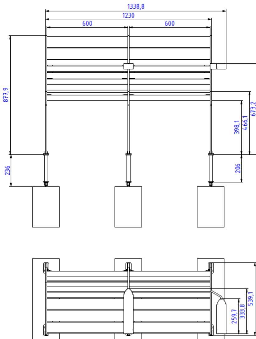
Fig. 2-seater version dimensions
